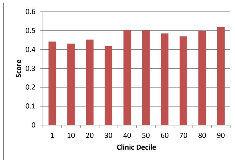
Figure 13: Day 5 Mean Embryo Score by Clinic Decile
